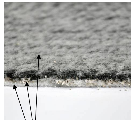
Geotextil PP woven 130 g/m 2 Bentonit granulat 5000 g/m 2 Geotextil PP nonwoven 200 g/m 2
