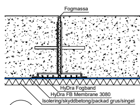
5A Dilatationsfog EXT
