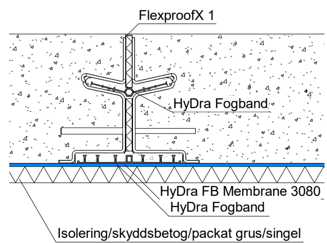
5B Dilatationsfog EXT/INT
